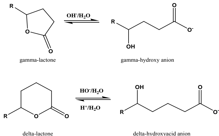
Figure III.1. Equilibrium of gamma- and delta-lactone and hydroxycarboxylate anion.
