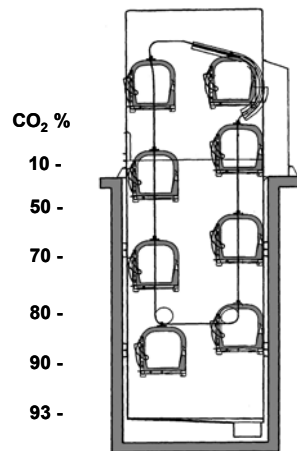
Figure 9-4. Principles in the carbon dioxide gradient in a paternooster carbon dioxide stunning system
